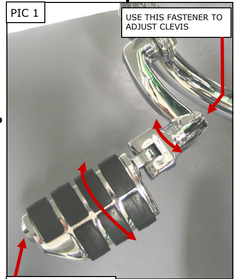
PIC 1 USE THIS FASTENER TO ADJUST CLEVIS USE THIS FASTENER TO ADJUST PEG
